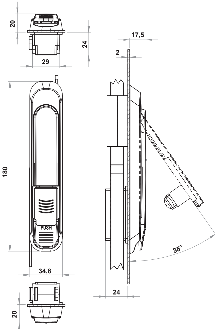
2307 - Swinghandle (Handle Zinc die, Plastic Housing)
