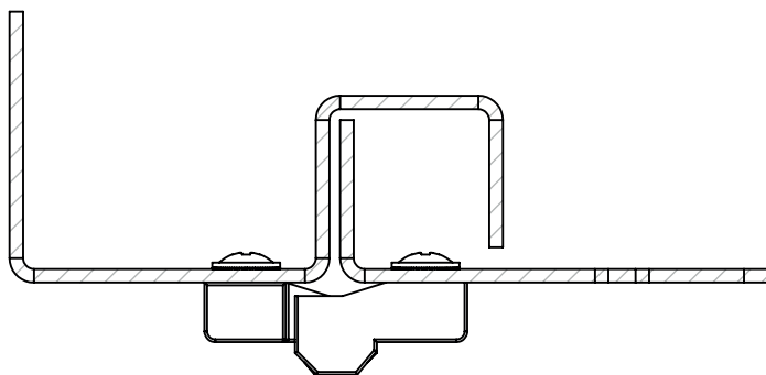
3059 - 180° Lift-off Hinge
