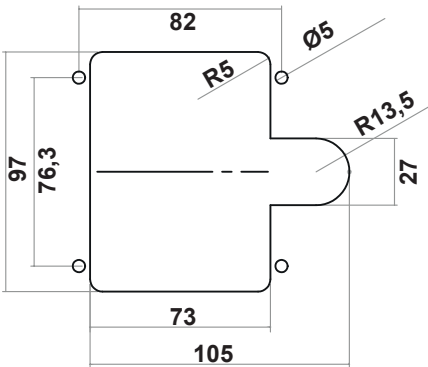
7634 - Cabinet Lock with T-Handle and Fixed Cam Grip range (H) : 60mm
